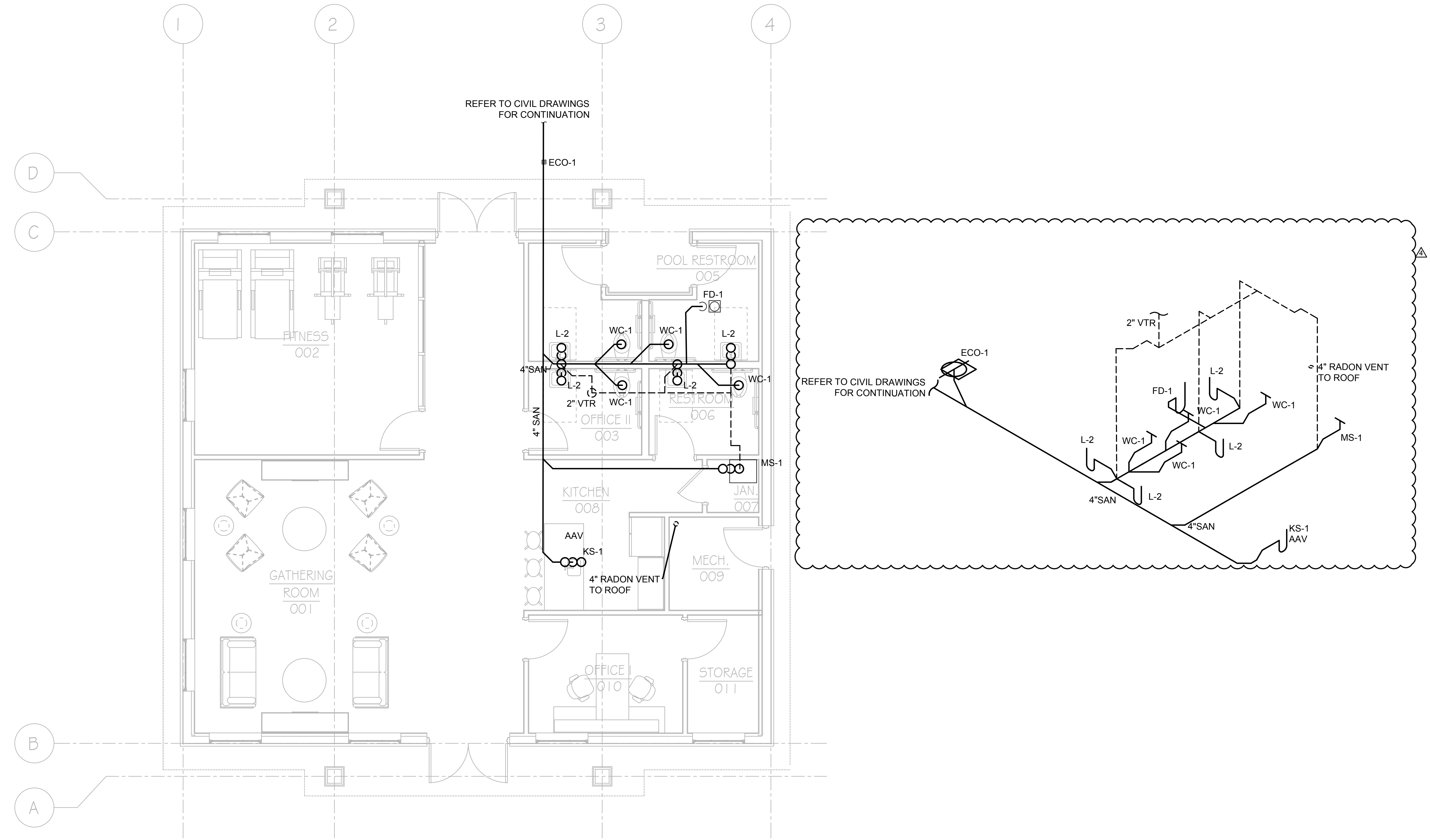
1 PLUMBING PLAN CLUBHOUSE GRAVITY SCALE: 1/4" = 1'-0"
